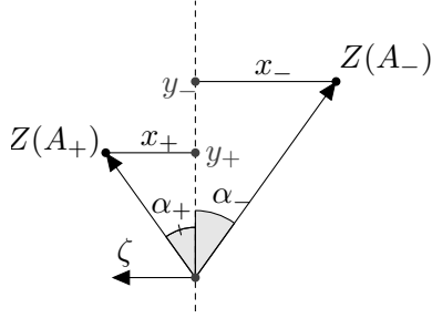
FIGURE 3. Computing the derivative v(\sigma).w_E
